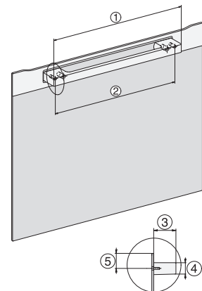
H7000 handle, installation drawing 1) 400 mm, 2) 360 mm, 3) 47 mm, 4) 24 mm, 5) 32.5 mm
