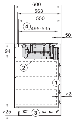
KMDA7272FR, KMDA7473FR – Side view lying on top, Plug&Play – Installation drawing
