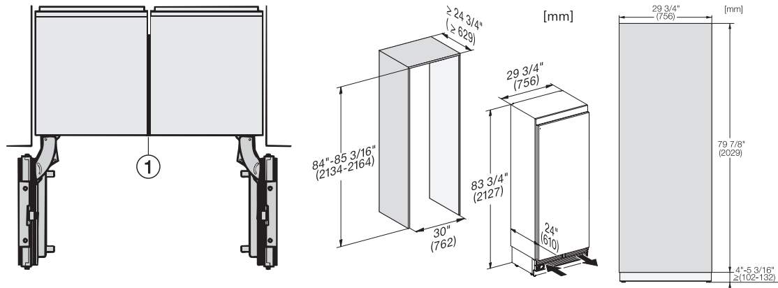
Side-by-side, MasterCool, without partition wall, with heating mat (Sketch) (with footnote)
